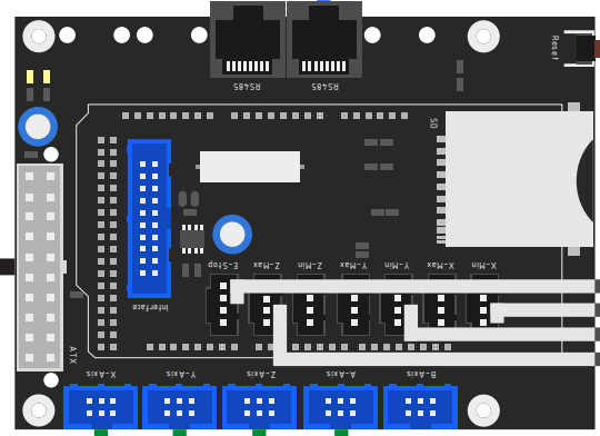
Motherboard
