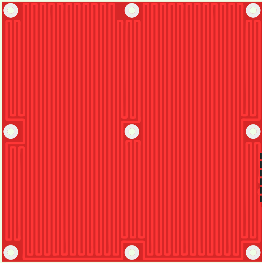
Heater Board
