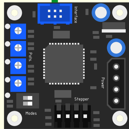
Y-Axis Controller
